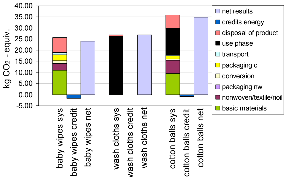
Figure: Key contributing life cycle stages for baby wipes, wash cloth and cotton wool balls (example given for global warming potential).
